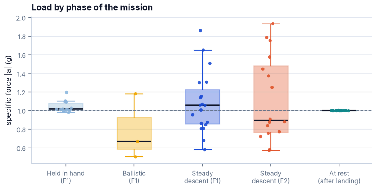
Figure 37 · The load on the vehicle by phase of the mission, in units of g: held in hand, ballistic, steady descent (both flights) and at rest after landing. The resting value (1.000 g, \sigma 0.0015 g) is the accelerometer's calibration made visible.
