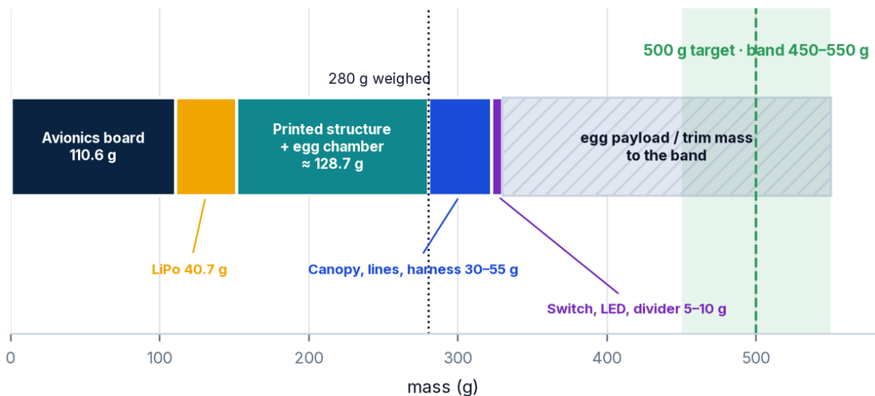
Figure 13 · From weighed parts to the mass band. The electronics were weighed separately (110.573 g board, 40.726 g battery); the 280 g bare vehicle was weighed after assembly; the structure is the difference.
