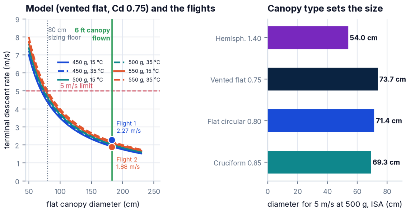
Figure 16 · Left: terminal descent rate against flat canopy diameter for the three masses of the band, on a standard day (solid) and a 35 °C day (dashed). The 80 cm sizing floor and the 6 ft canopy flown are marked, with the two measured flight rates. Right: the diameter needed for 5 m/s at 500 g for each canopy type.
