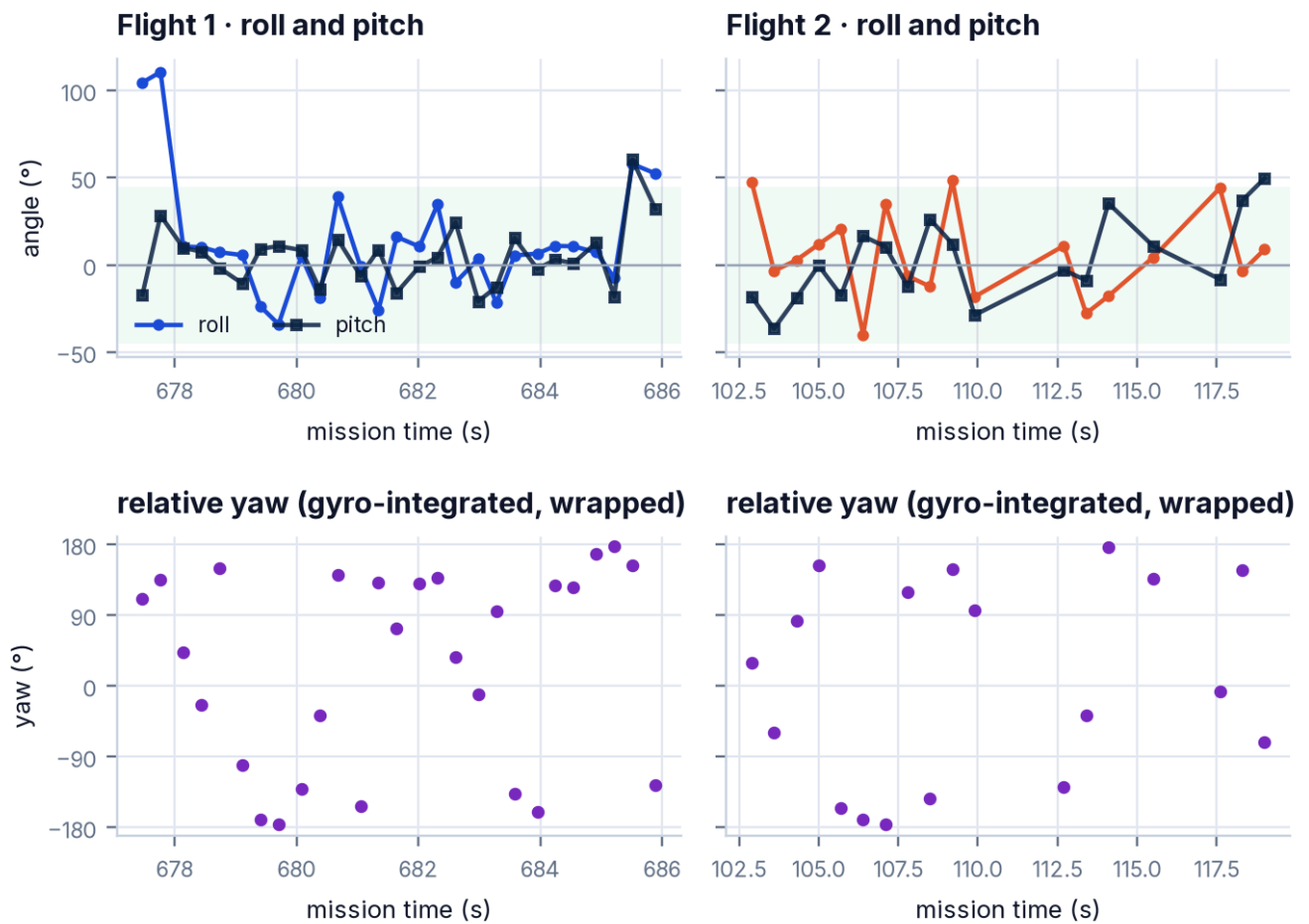
Figure 38 · Roll and pitch (top) and relative yaw (bottom) for both flights. Flight 1 starts at the throw, when the vehicle rotates from the orientation it was held in (roll \approx 110^\circ ) to upright within a packet.
