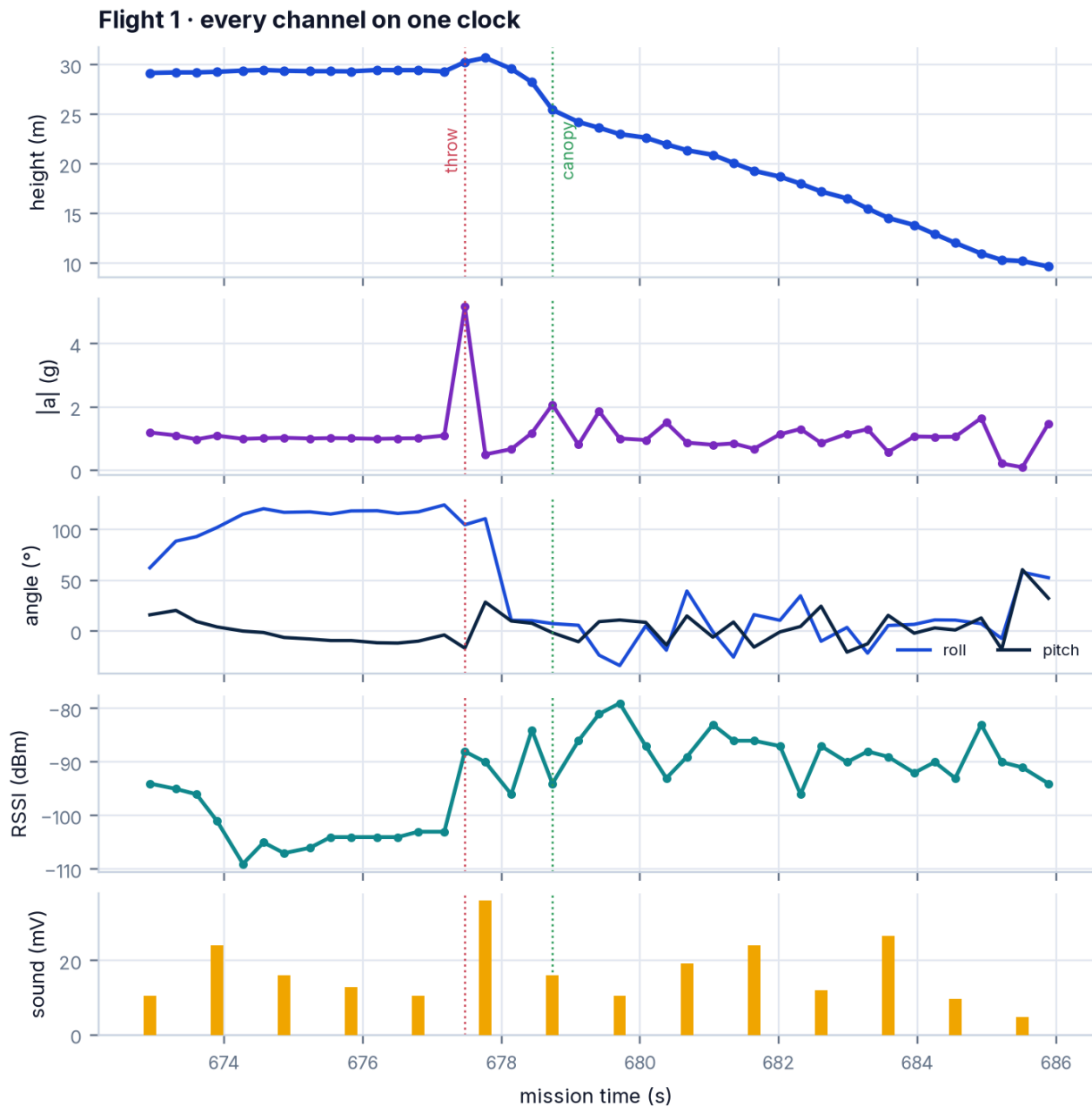
Figure 33 · Flight 1 on one clock. Height, specific force, roll and pitch, RSSI and acoustic level — the throw and the canopy opening marked. The same instant shows up in every channel: the acceleration spike, the roll swinging from 110° (on its side) to upright, the radio signal improving by 14 dB, and the loudest microphone packet.
