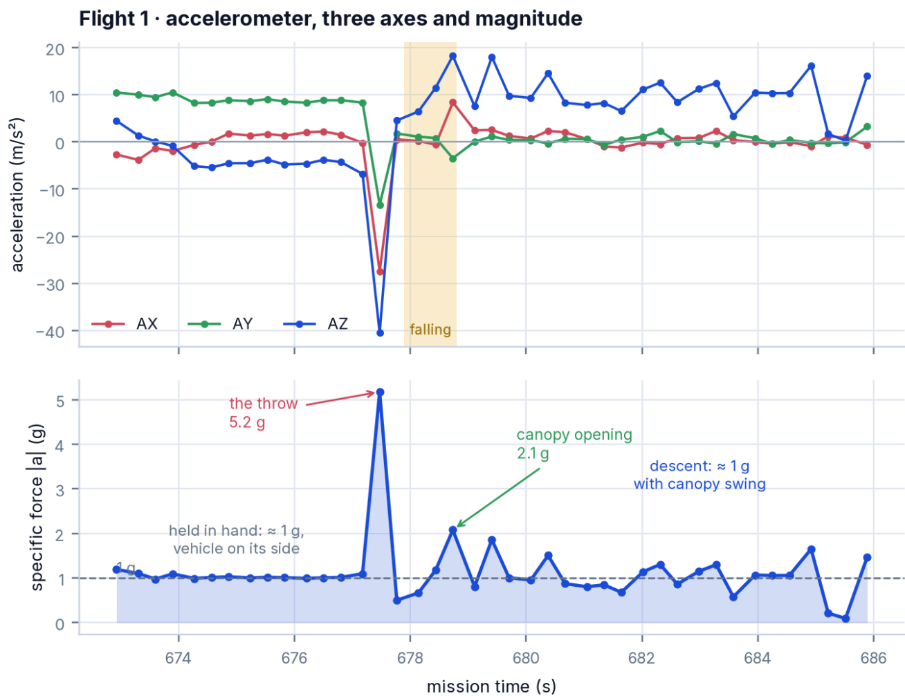
Figure 32 · Flight 1 — acceleration. The throw (5.2 g), the dip below 1 g in the air, the canopy-opening load (2.1 g) and the descent at about 1 g with canopy swing.
