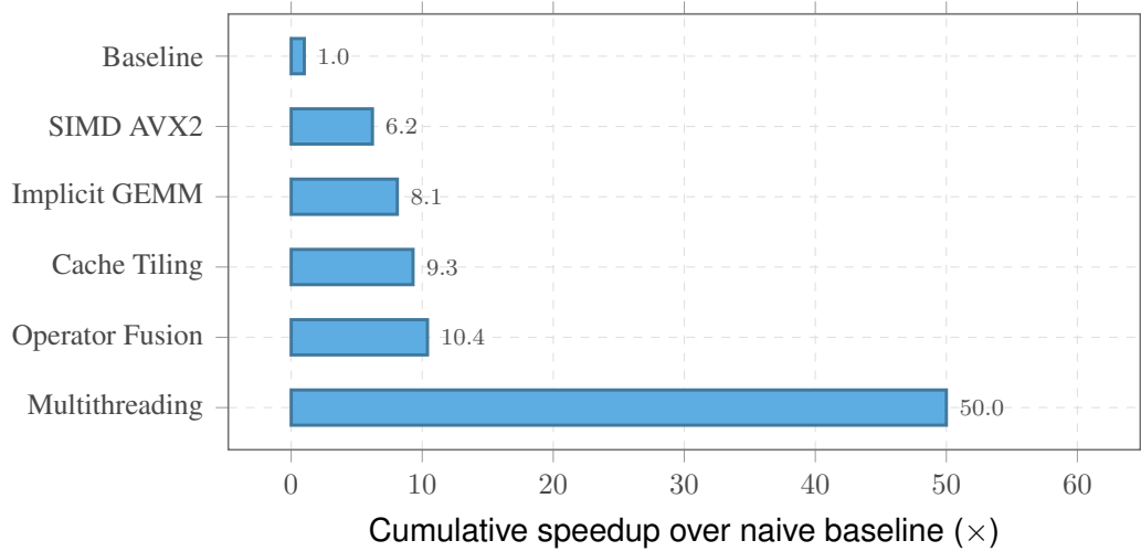
Figure 5.5: Cumulative speedup as each optimization is layered on. Effects are multiplicative; the combined stack reaches a significant speedup over a naive scalar convolution.
