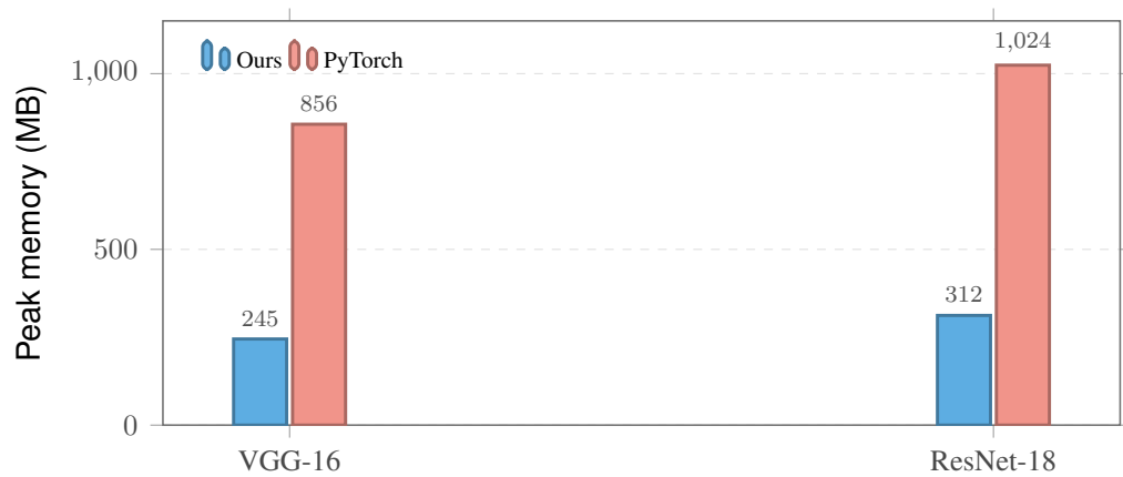
Figure 5.2: Peak inference memory. Eliminating im2col buffers and fusing \text{Conv} \rightarrow \text{BN} \rightarrow \text{ReLU} cuts memory by roughly 70%.
