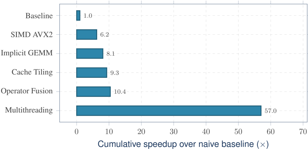
Figure 5.5: Cumulative speedup as each optimization is layered on. Effects are multiplicative; the combined stack reaches roughly 57\times over a naive scalar convolution.
