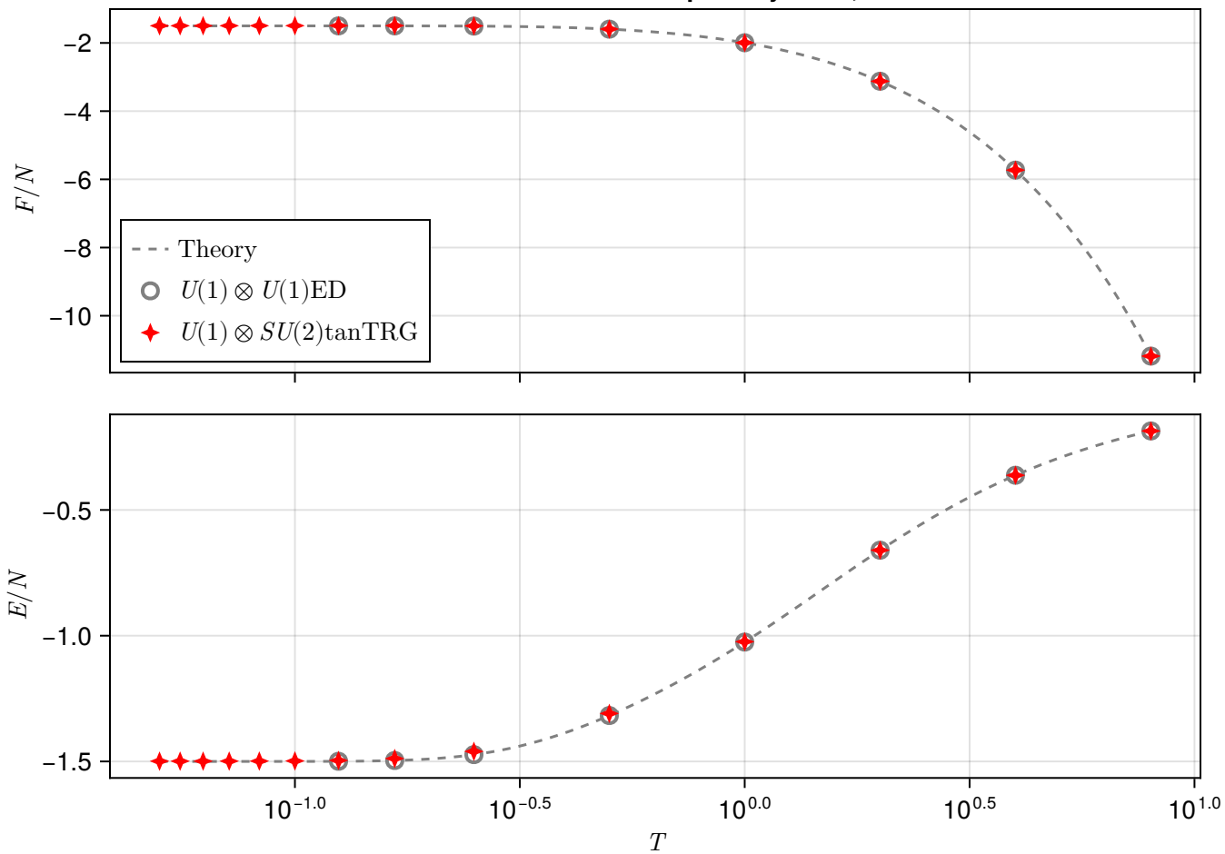
Hubbard model on 4x2 square cylinder, U = 0
