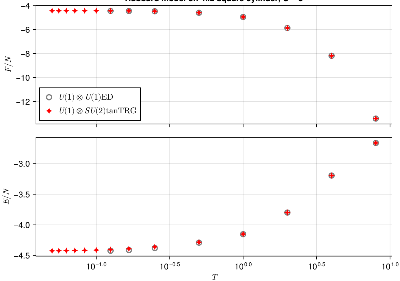
Hubbard model on 4x2 square cylinder, U = 8
