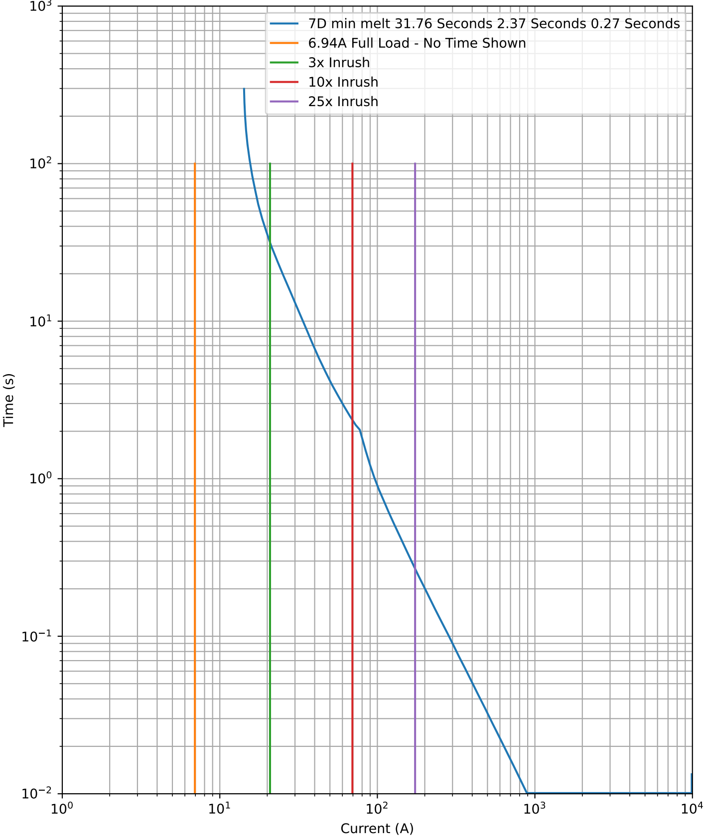
100kVA Time Coordination Chart
