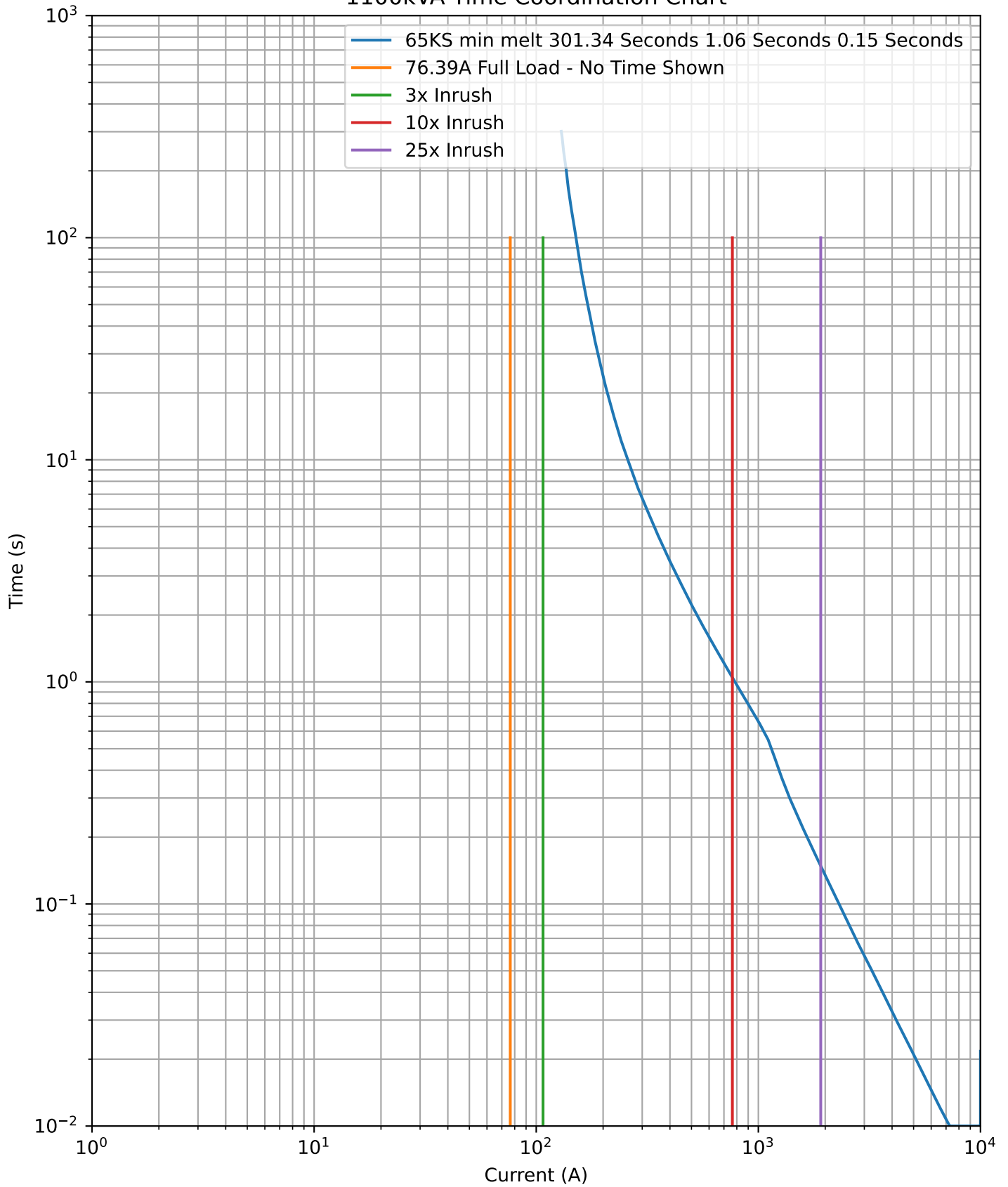
1100kVA Time Coordination Chart
