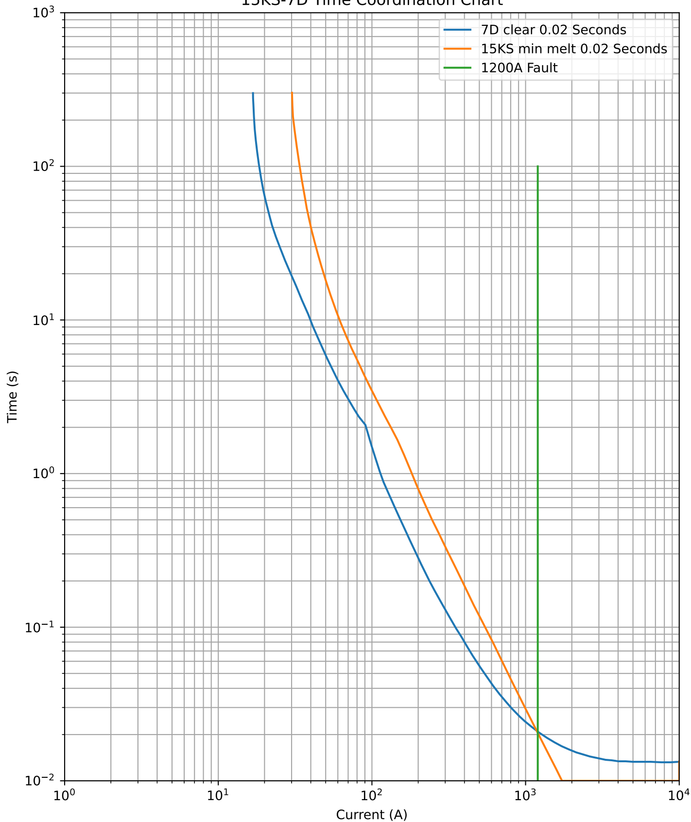
15KS-7D Time Coordination Chart
