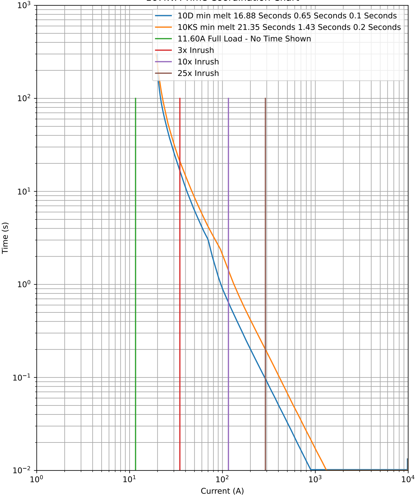
167kVA Time Coordination Chart
