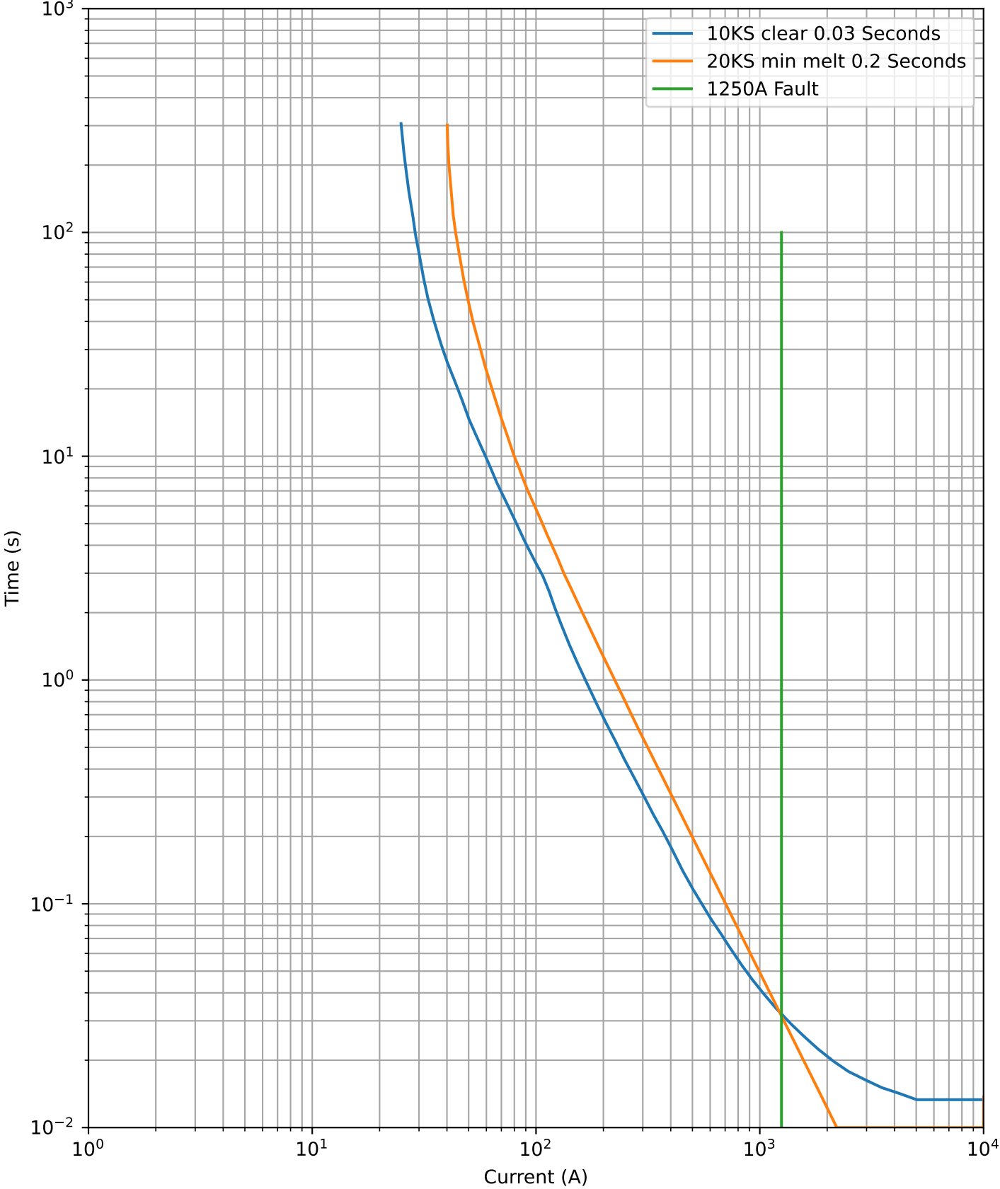
20KS-10KS Time Coordination Chart
