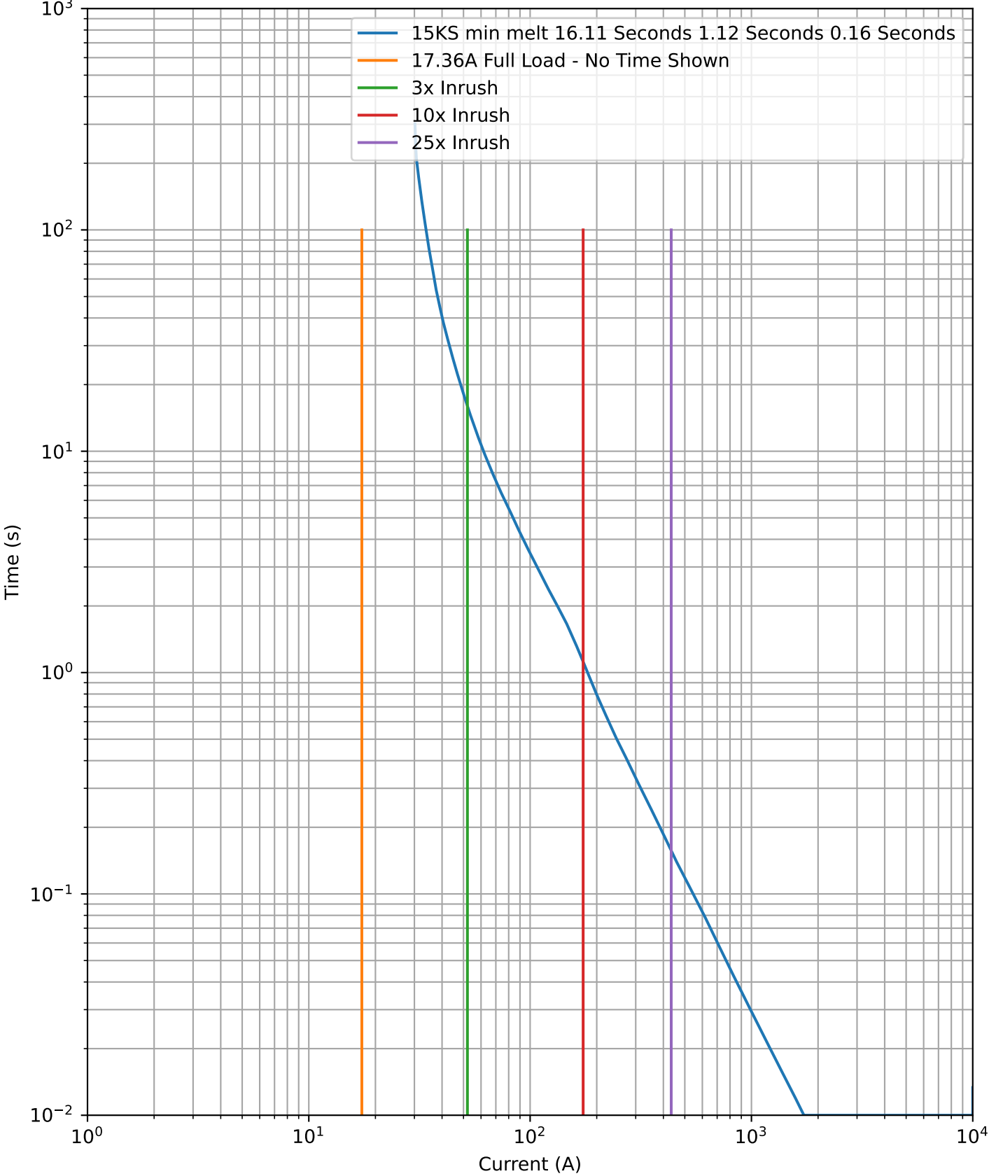
250kVA Time Coordination Chart
