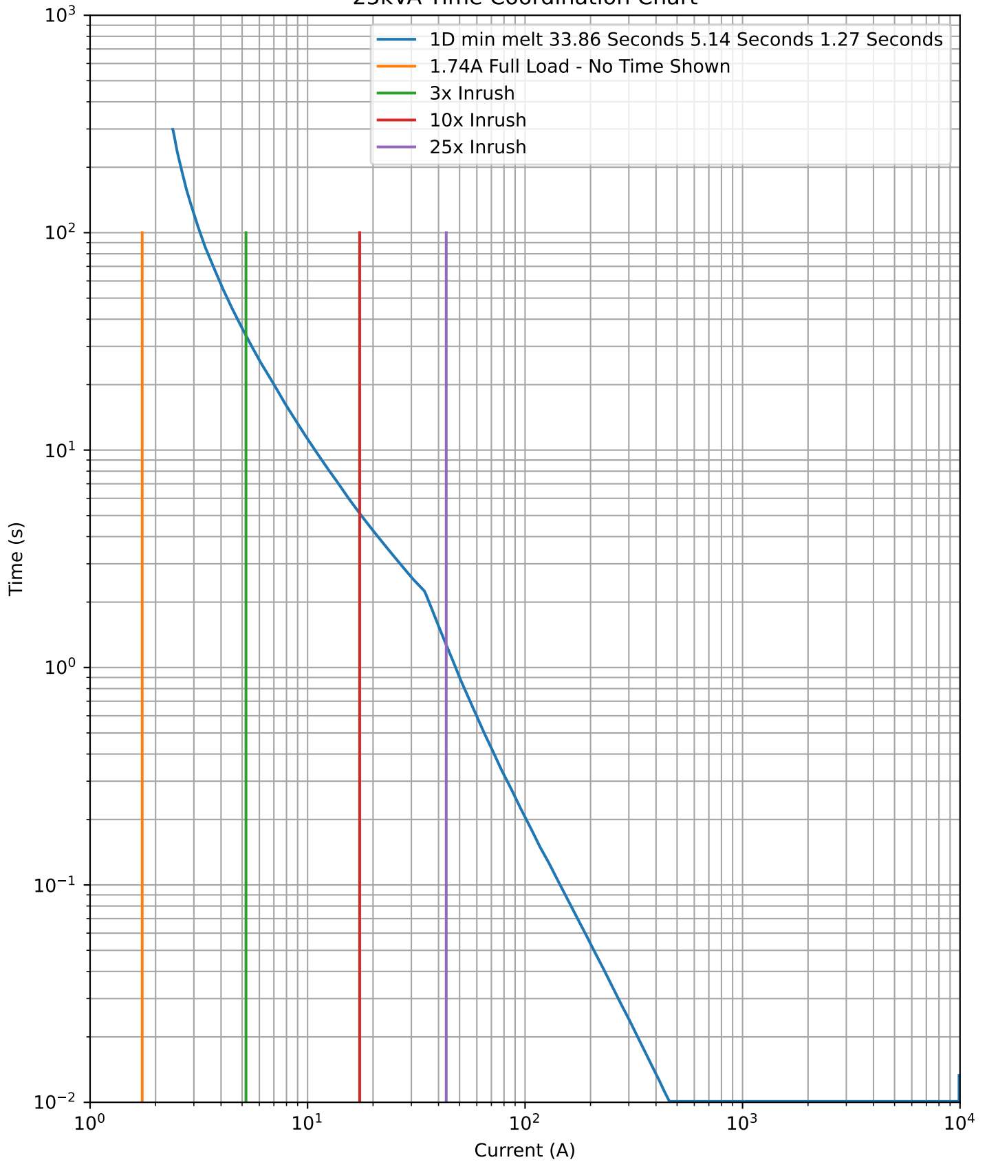
25kVA Time Coordination Chart
