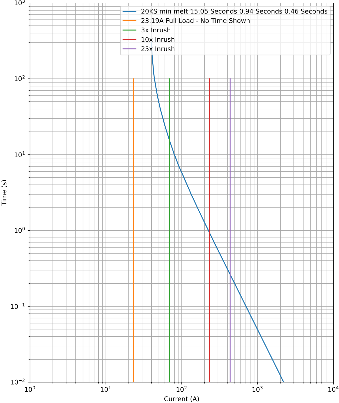
334kVA Time Coordination Chart
