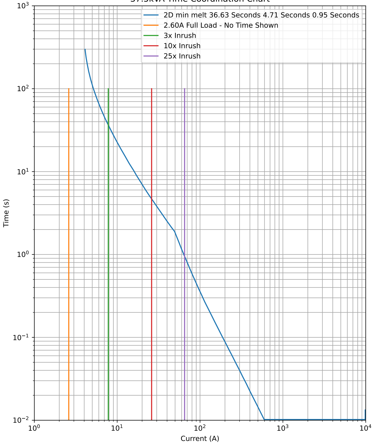
37.5kVA Time Coordination Chart
