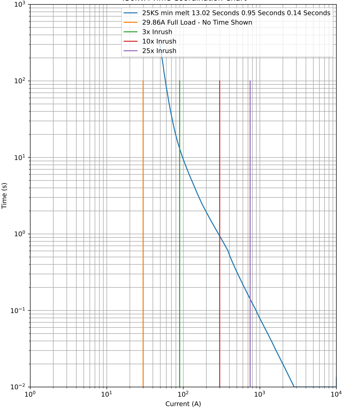
430kVA Time Coordination Chart
