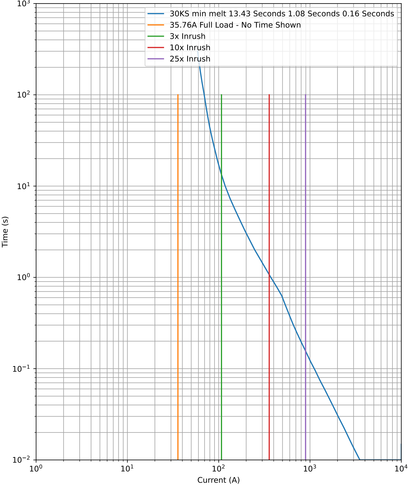
515kVA Time Coordination Chart
