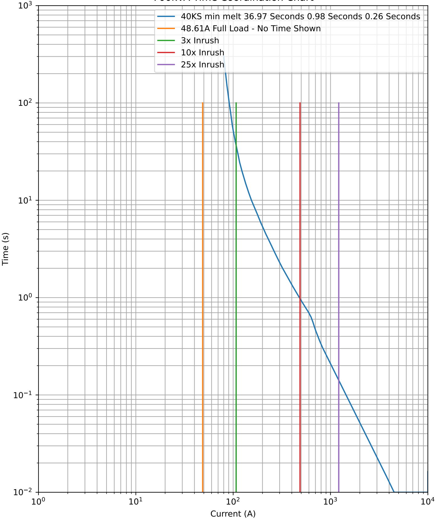
700kVA Time Coordination Chart
