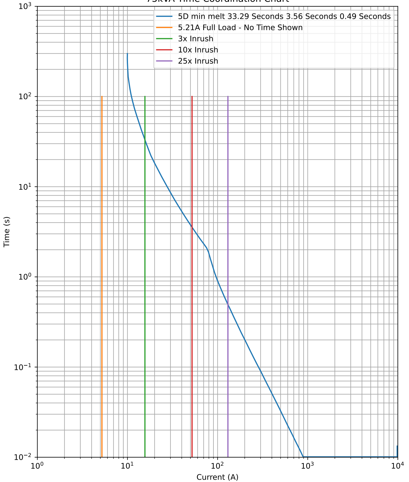
75kVA Time Coordination Chart
