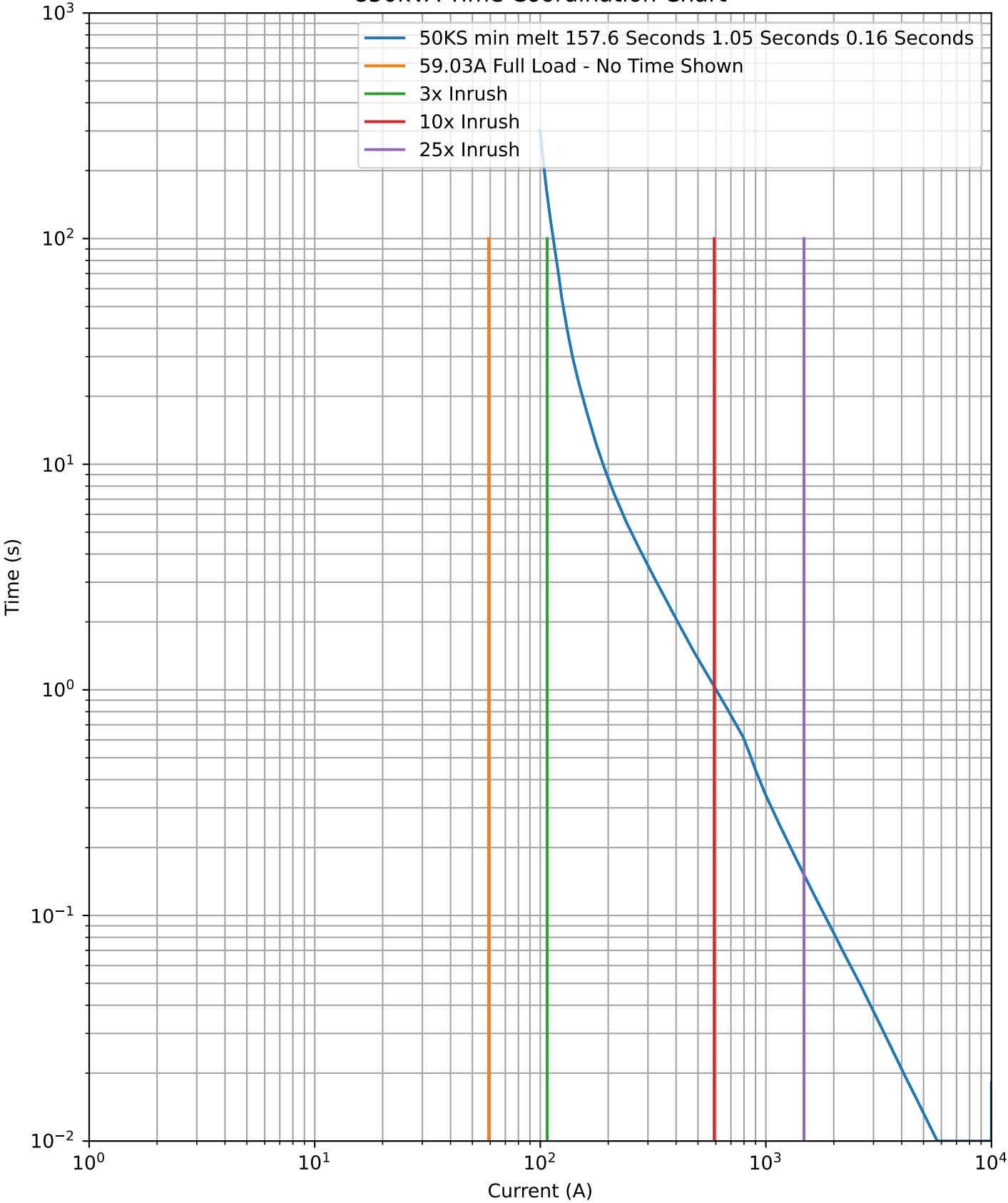
850kVA Time Coordination Chart
