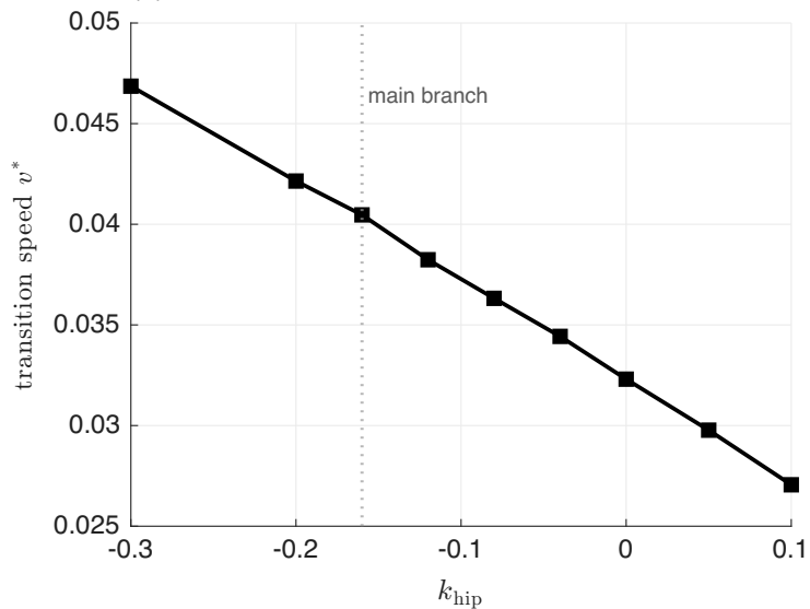
(b) where the mode switch occurs
