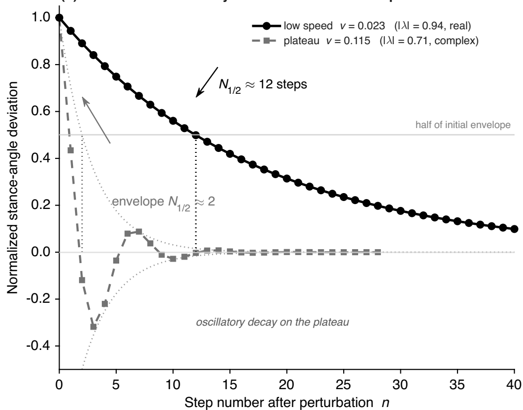
(b) Perturbation recovery is much slower at low speed
