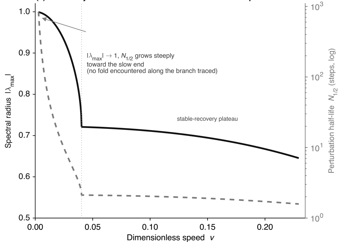
(a) Recovery weakens toward the slow end of the computed branch
