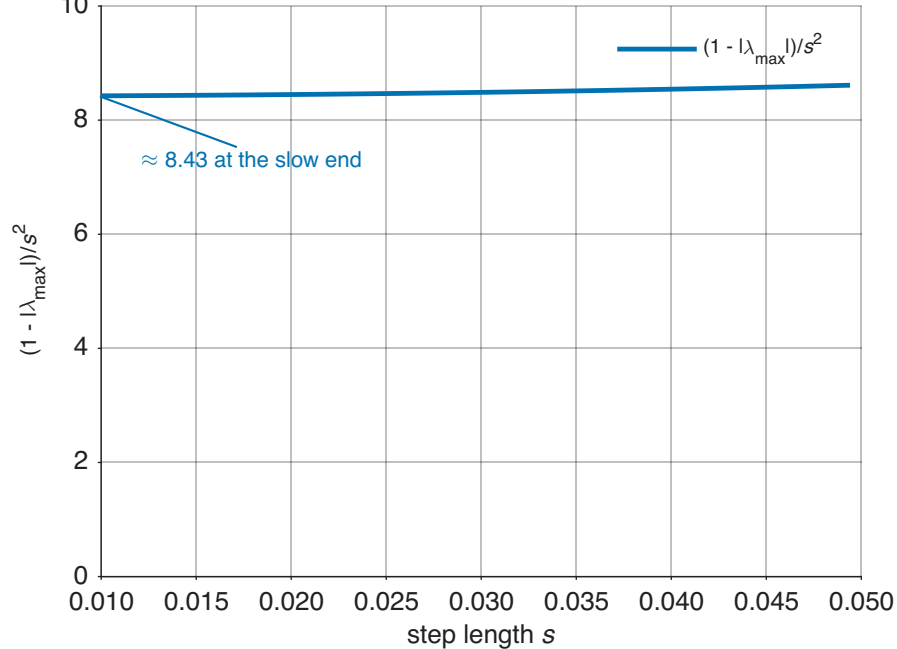
(b) local ratio approaches 8.43 at low s
