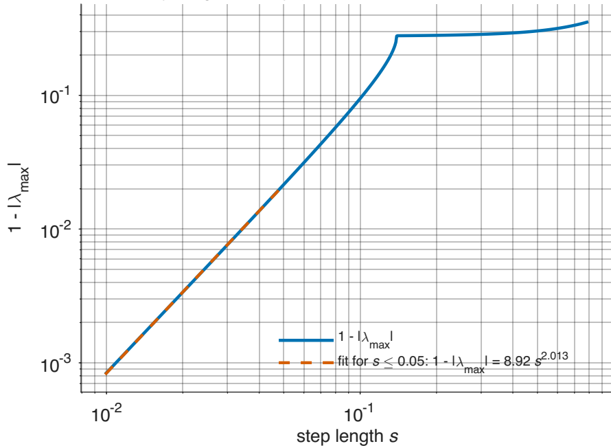
(a) recovery margin is nearly quadratic at low s
