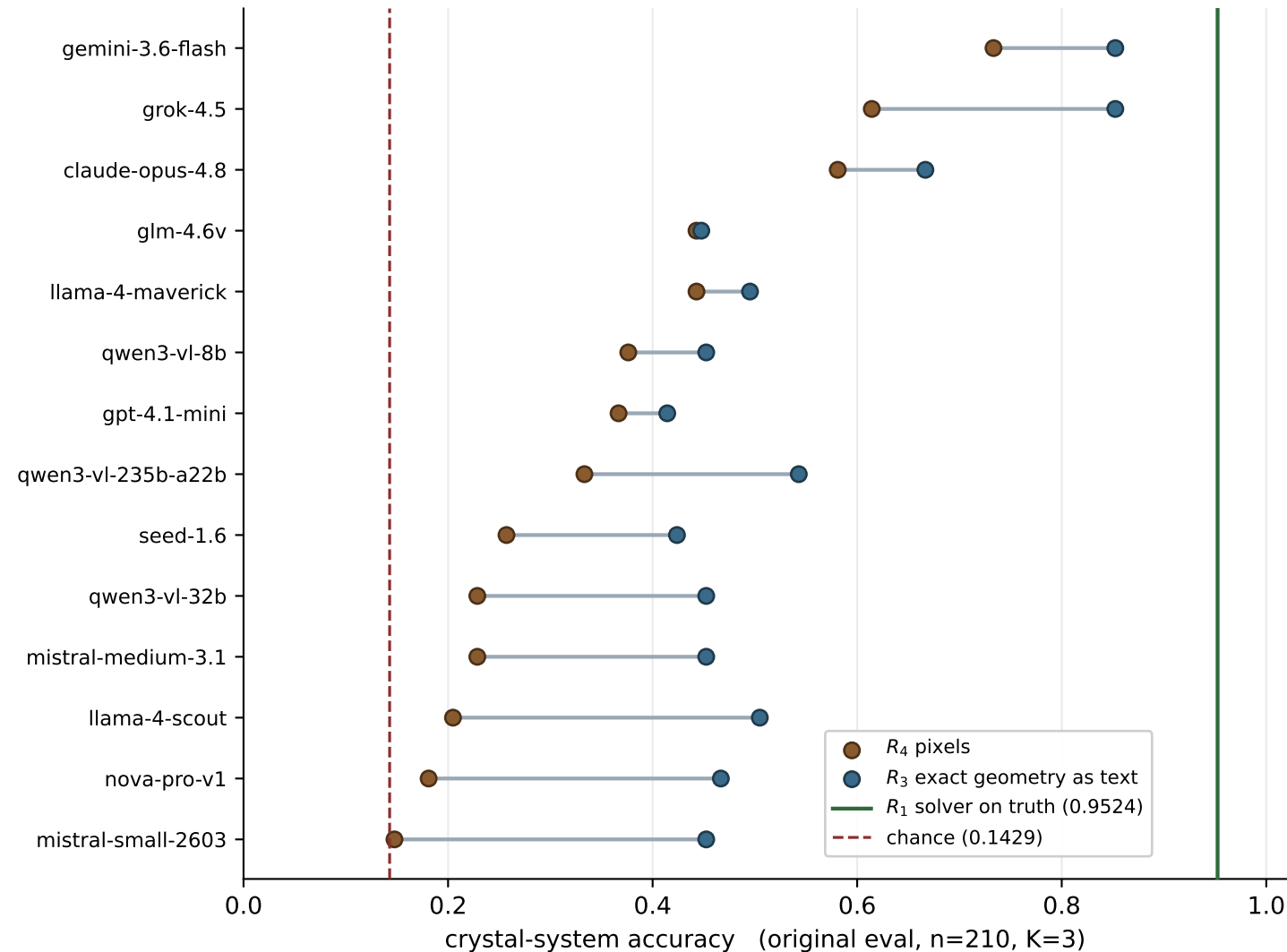
Supplying exact geometry does not close the gap to the solver
