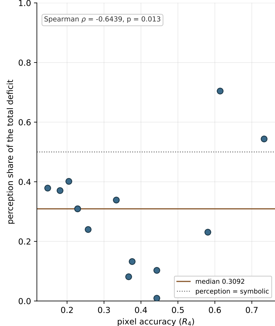
The bottleneck moves with model strength
