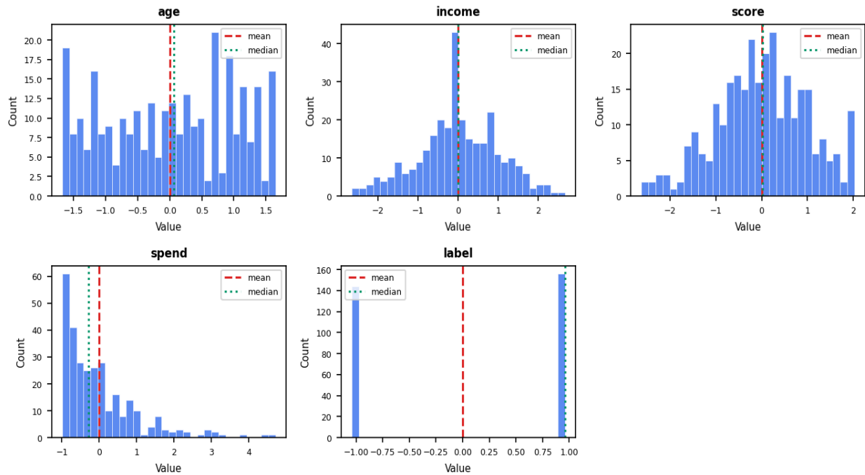
Feature Distributions
