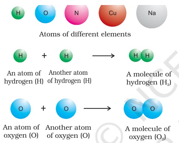
Fig. 1.3 A representation of atoms and molecules
