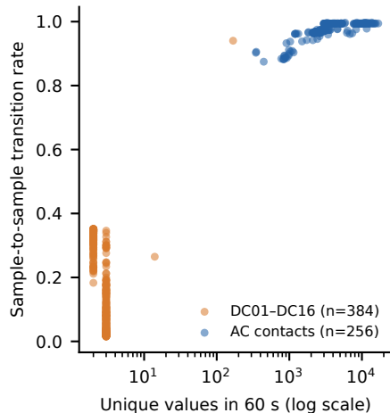
b AC contacts: continuous signals
