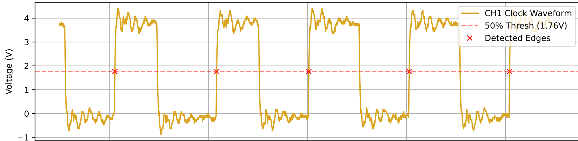
Tektronix TDS 2001C — SPI Clock Waveform
