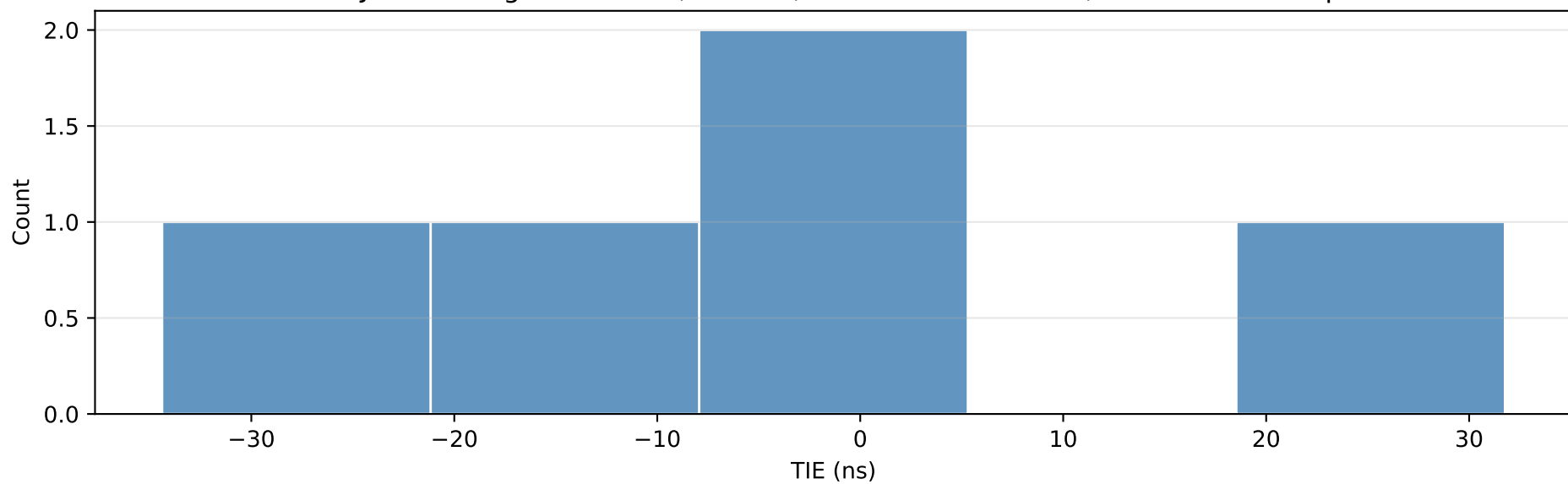
TIE Jitter Histogram — N=5, Bins=5, Mean=-4.011905 ns, Std=21977.104 ps
