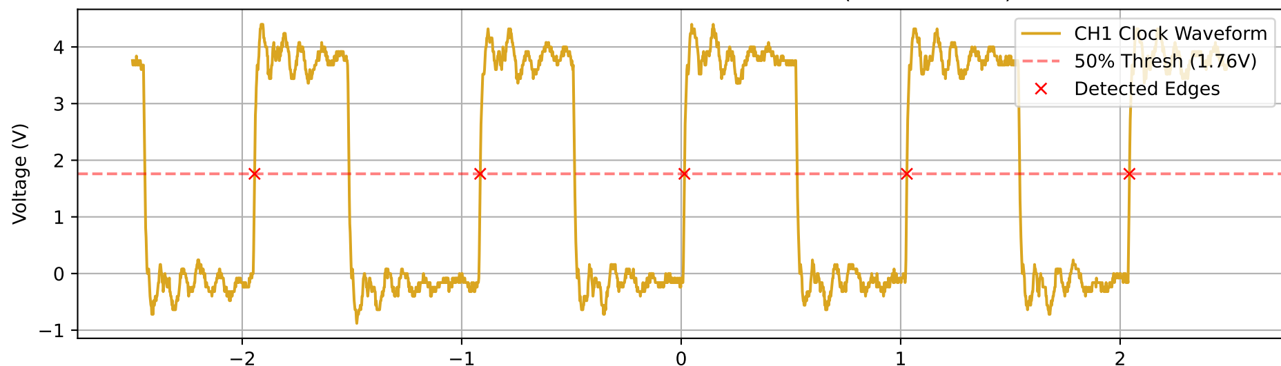
Tektronix TDS 2001C — SPI Clock Waveform (1003.440 kHz)
