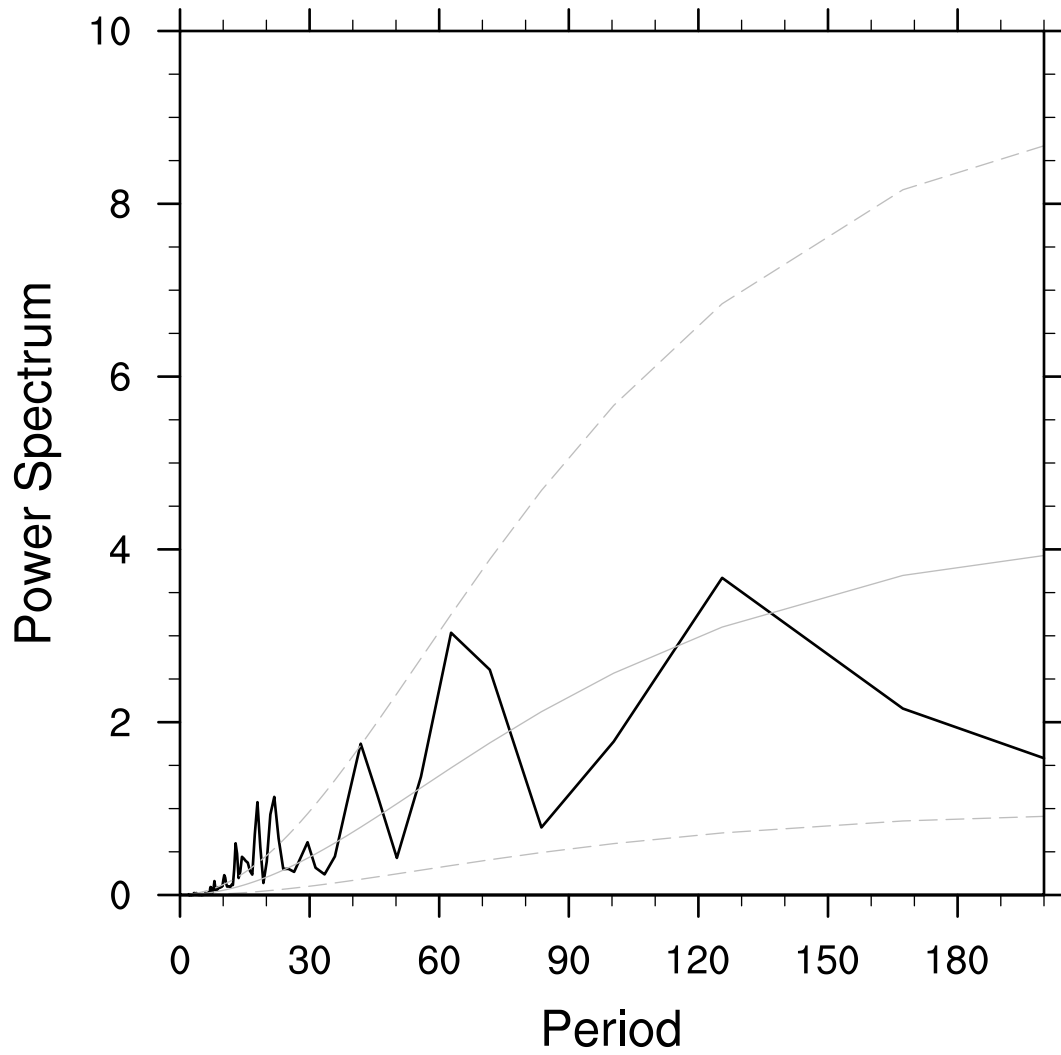
Power Spectrum of Sea Ice Timeseries
