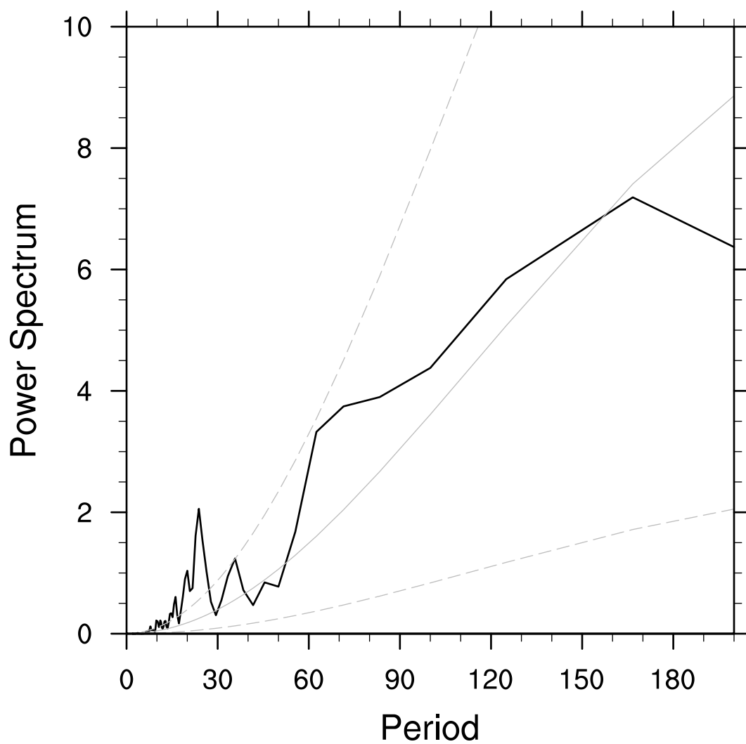
Power Spectrum of Sea Ice Timeseries (ESM2M)
