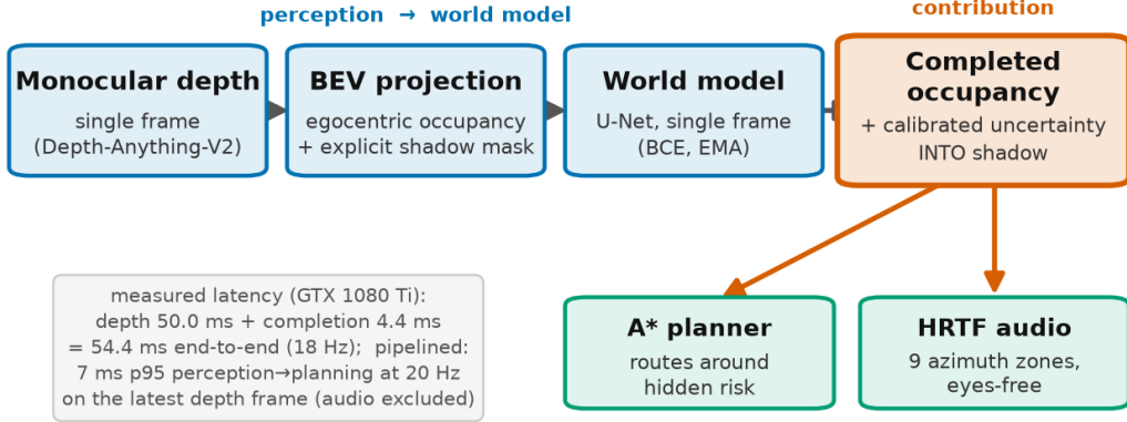
Figure 1: ShadowWeave pipeline. A single monocular-depth frame is lifted by a differentiable projector into an egocentric 96 \times 96 BEV occupancy grid together with a visibility grid; thresholding visibility yields the explicit shadow mask marking cells the sensor cannot see. A 31M-parameter U-Net predicts per-cell occupancy probabilities at 1/3/5/10 s horizons inside that mask; the completed grid and its uncertainty feed an A* planner and a nine-zone HRTF spatial-audio interface for eyes-free navigation.
