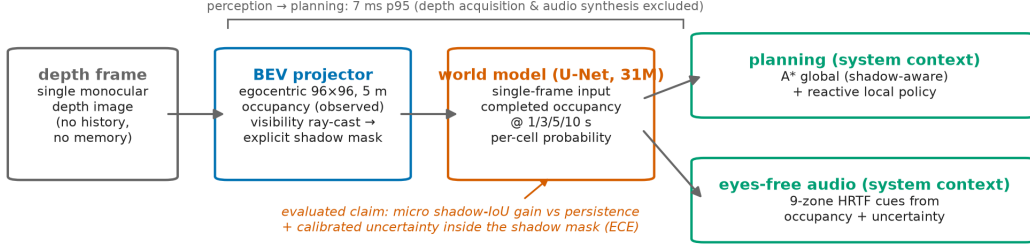
Figure 1: ShadowWeave pipeline. A single monocular-depth frame is lifted by a differentiable projector into an egocentric 96 \times 96 BEV occupancy grid together with a visibility grid; thresholding visibility yields the explicit shadow mask marking cells the sensor cannot see. A 31M-parameter U-Net predicts per-cell occupancy probabilities at 1/3/5/10 s horizons inside that mask; the completed grid and its uncertainty feed an A* planner and a nine-zone HRTF spatial-audio interface for eyes-free navigation.
