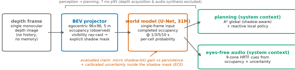
Figure 1: ShadowWeave pipeline. A single monocular-depth frame is lifted by a differentiable projector into an egocentric 96 \times 96 BEV occupancy grid together with a visibility grid; thresholding visibility yields the explicit shadow mask marking cells the sensor cannot see. A 31M-parameter U-Net predicts per-cell occupancy probabilities at 1/3/5/10 s horizons inside that mask; the completed grid and its uncertainty feed an A* planner and a nine-zone HRTF spatial-audio interface for eyes-free navigation.
