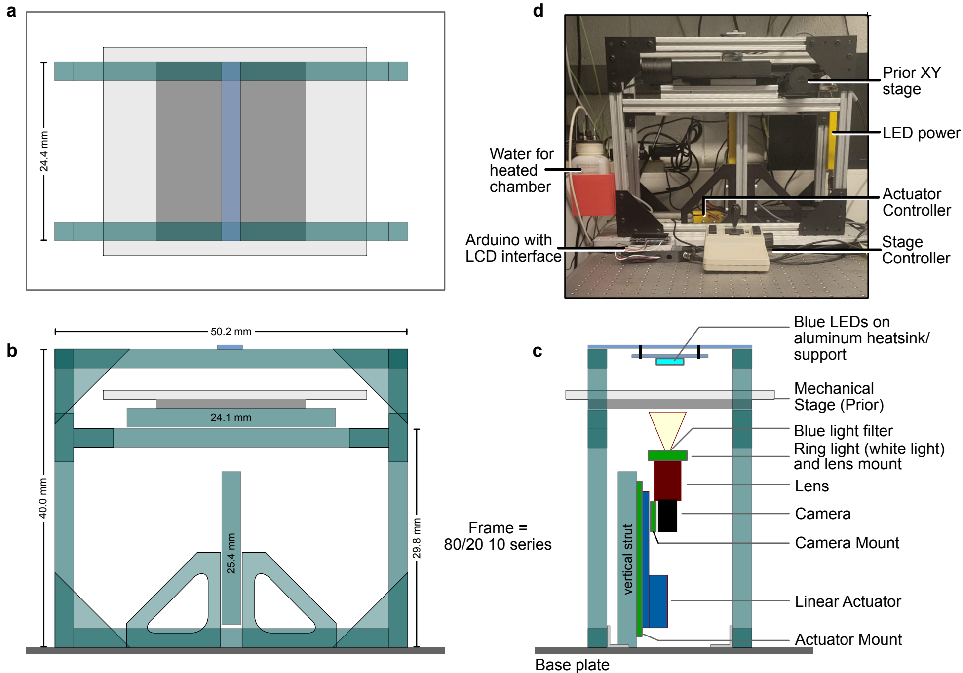
Figure 1. EHT assay device design. a-c. Schematic top (a), front (b), and side (c) views showing the 80/20 extruded aluminum frame supporting the mechanical stage. The side view details the camera attachment to a linear actuator through 3D printed mounts. A 3D printed attachment to the top of the lens holds a white LED ring light and a blue long-pass filter. The blue pacing LEDs are mounted above the stage under an aluminum heatsink/support. d. EHT assay device photo taken from the front.
