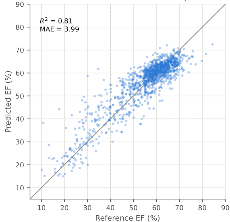
(b) Recommended: R3D-18 32f×p2
