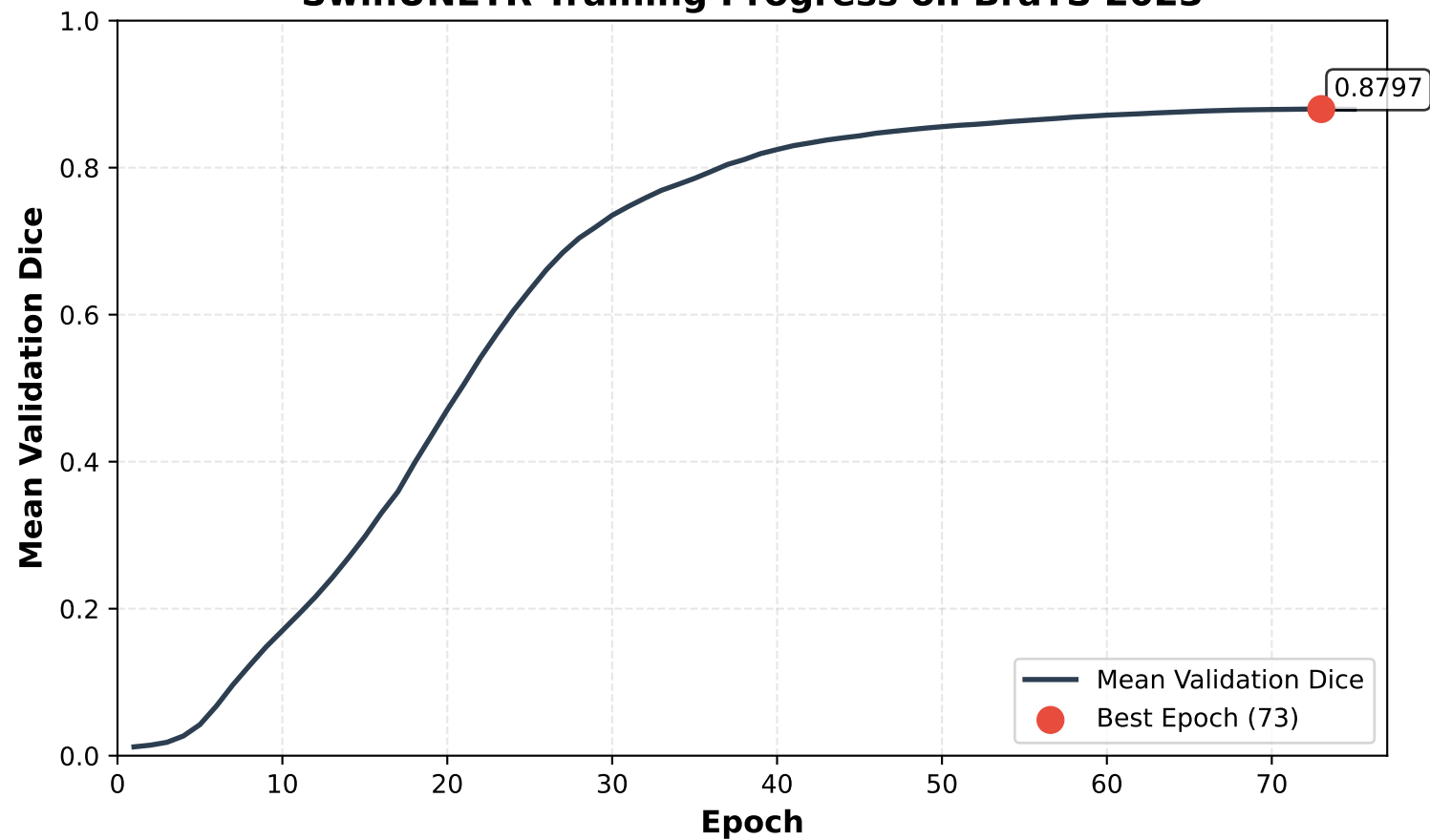
SwinUNETR Training Progress on BraTS 2023
