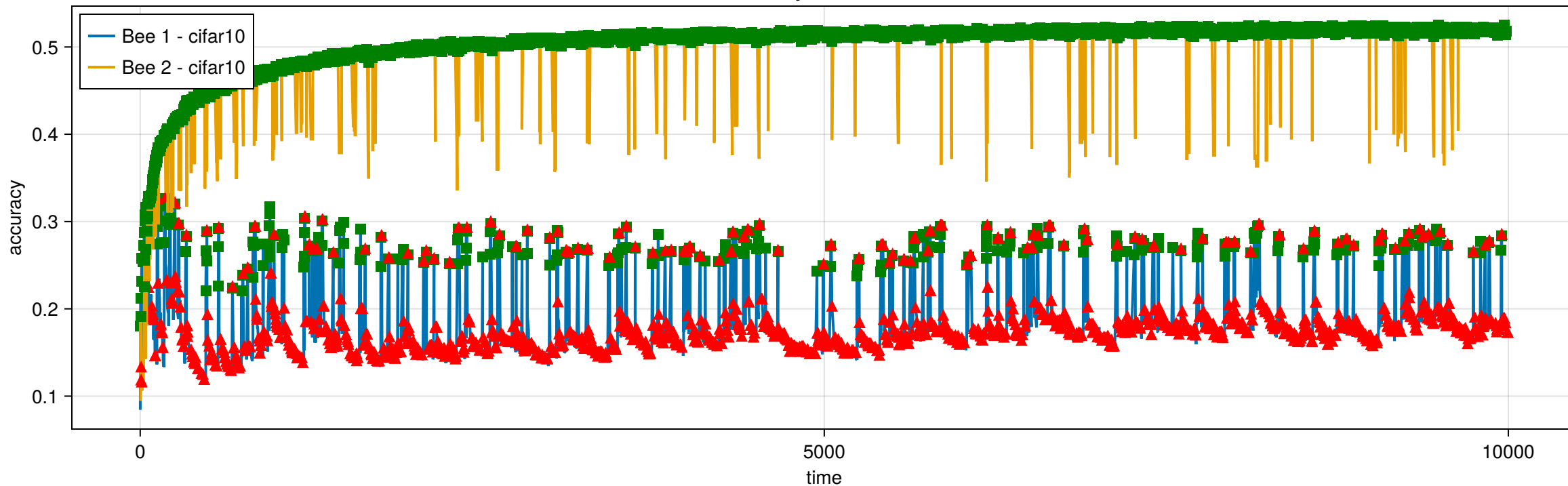
Evolution of Accuracy for Task 1 across all Bees
