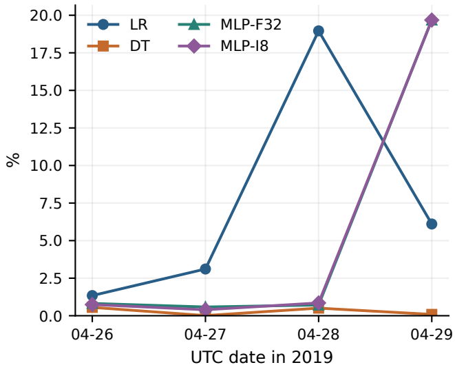
(a) Daily false-positive rate
