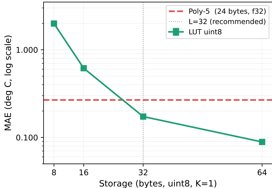
Accuracy-memory Pareto frontier (NTC)
