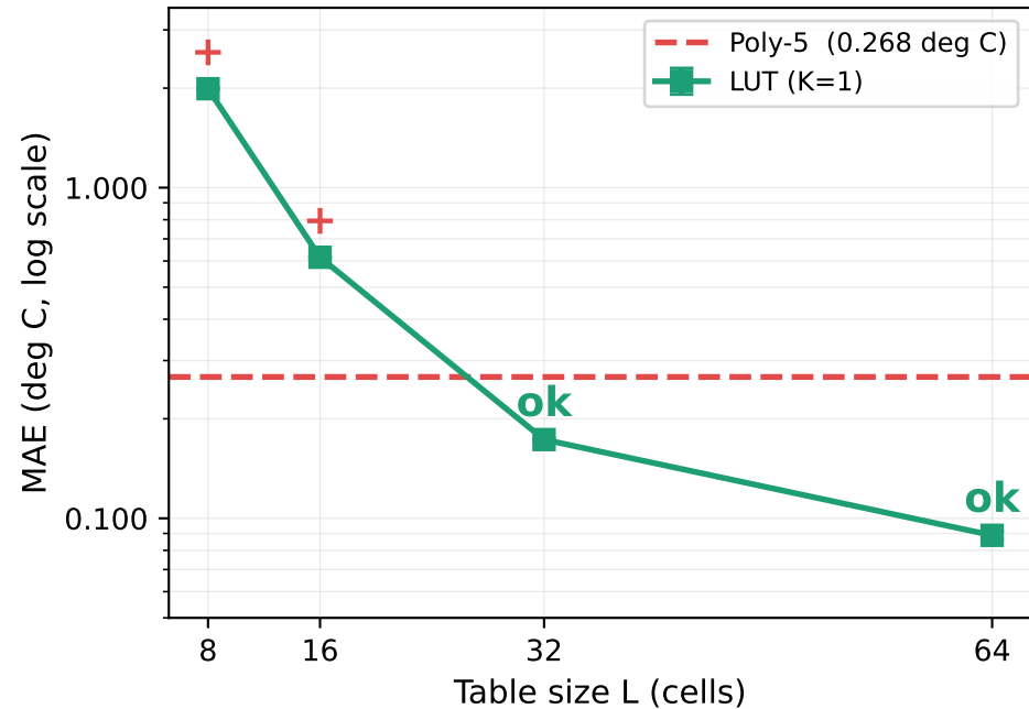
NTC: LUT accuracy vs. table size
