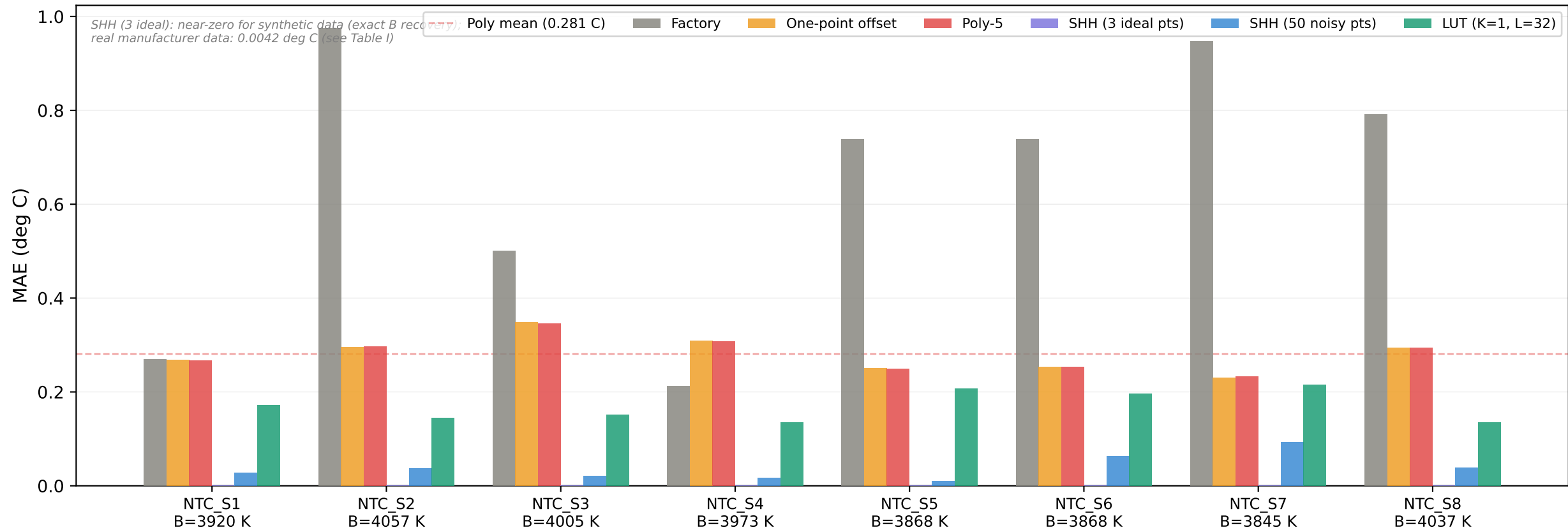
NTC thermistor: all calibration methods (50 noisy cal. points, K = 1 , L = 32 , 5 seeds)
