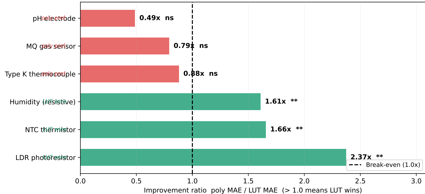
Regime map: LUT vs. polynomial calibration ( K = 1 , L = 32 , N_{\text{cal}} = 50 )
