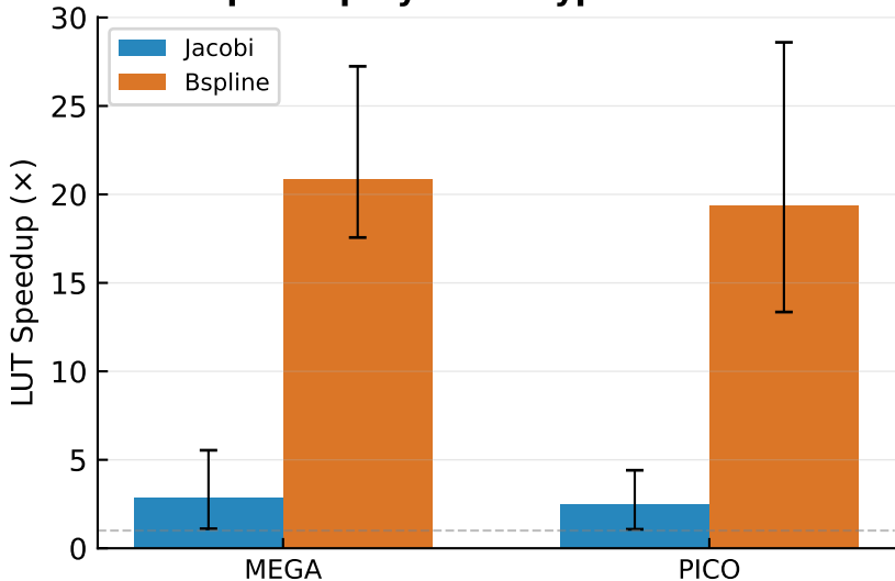
LUT Speedup by Basis Type and Platform
