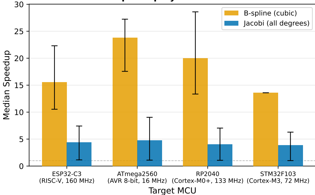
LUT-KAN Speedup by Basis and Platform
