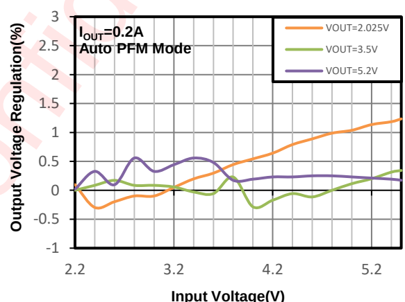
Output Voltage Regulation vs Input Voltage
