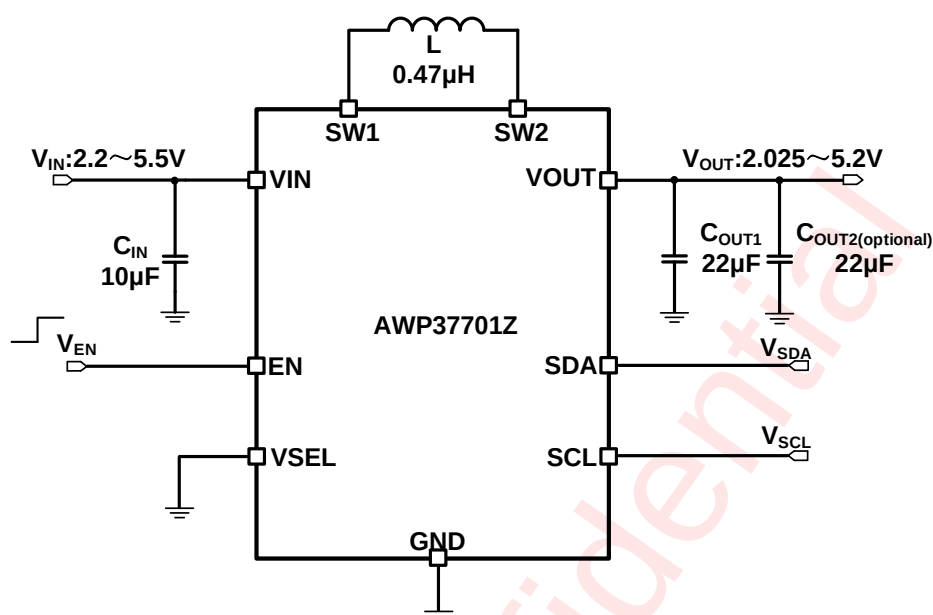
Figure 4 AWP37701Z Typical Application Circuit
