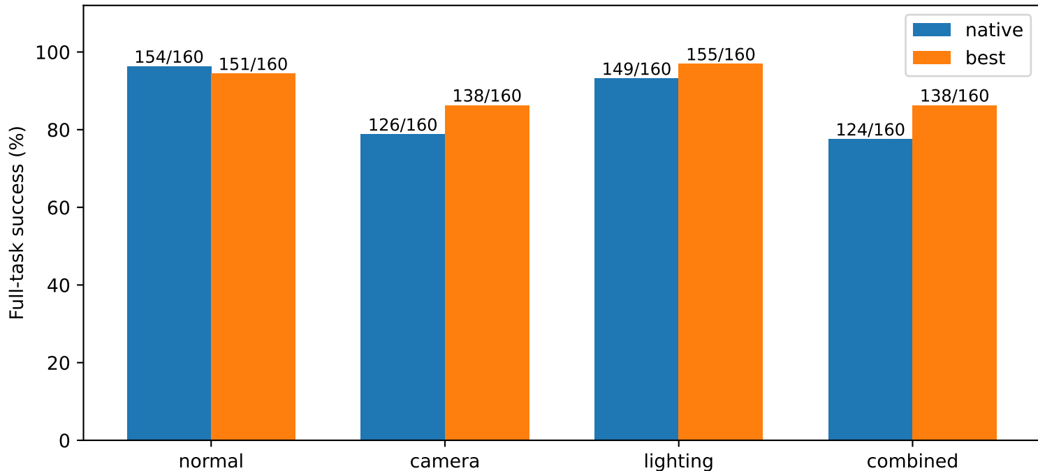
Stage 1 best vs native: all 40 LIBERO source tasks
