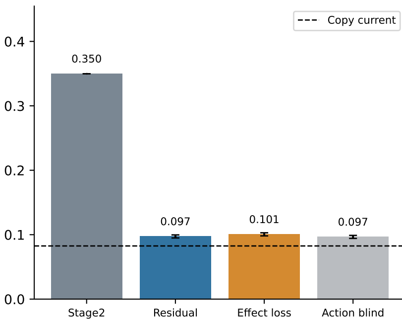
Future-feature error (lower better)
