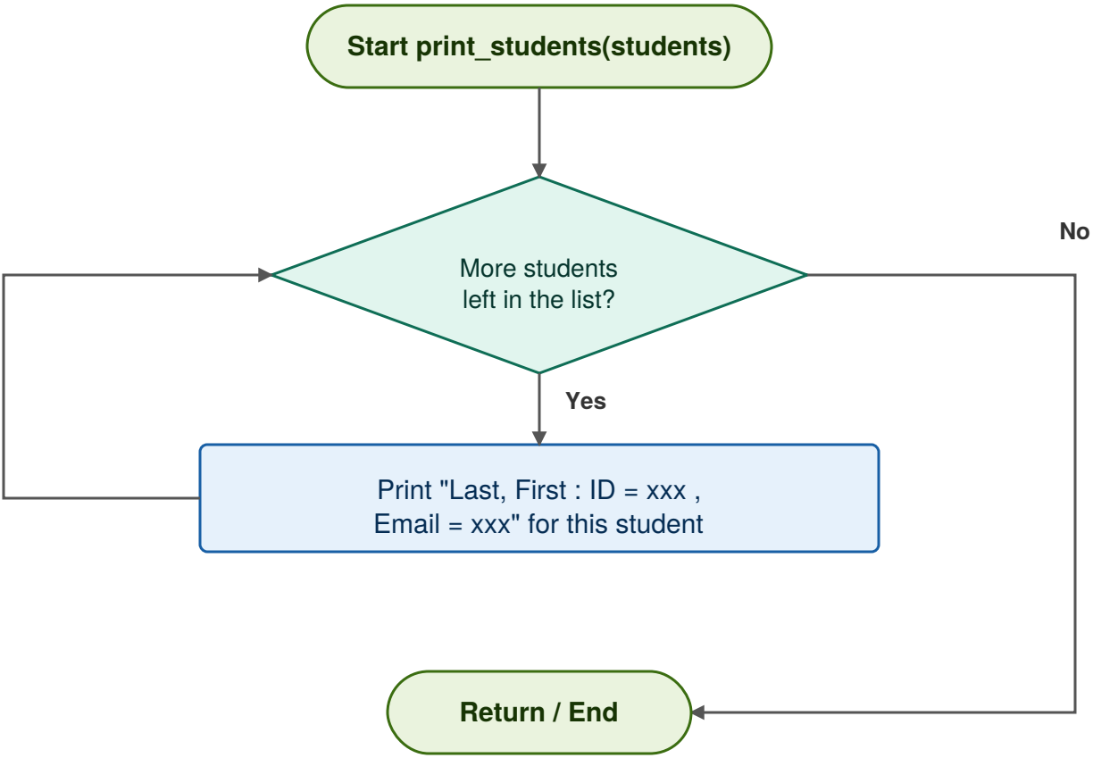
Diagram 2: print_students(students) subprocess
