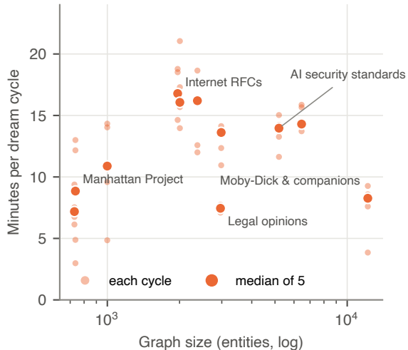
(b) Dream cycle, 200-completion budget
