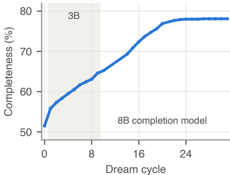
(a) Graph completeness
